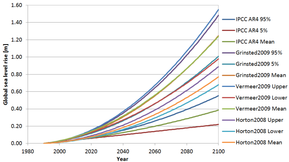
Figure 3.2 Global sea level rise for the various models for the emission scenario A2
