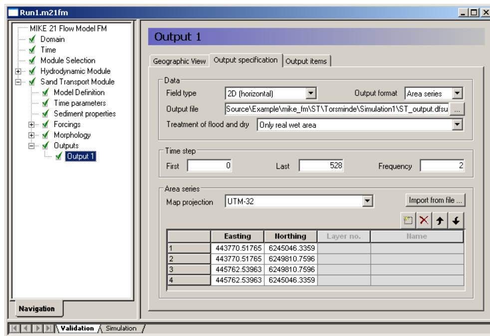
Figure 4.24 MIKE 21 Flow Model FM, Sand Transport Module: Output type and location
