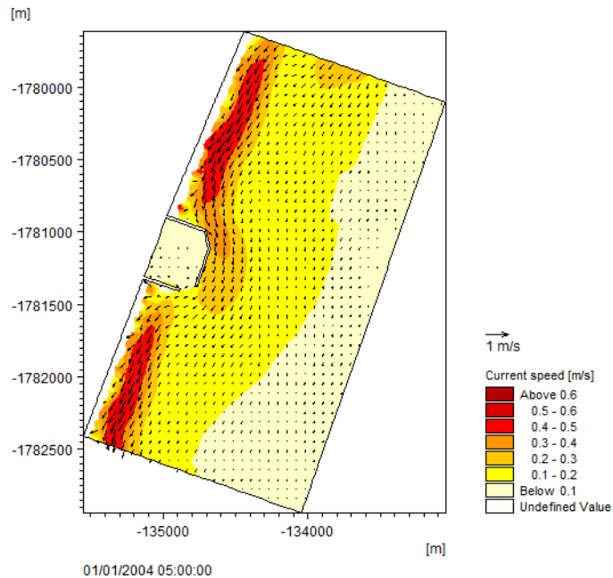
Figure 4.15 Contour and vector plot of the flow field.
