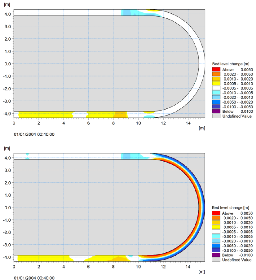
Figure 4.4 Contour plot of bed level change after 40 minutes. Upper figure: excluding helical flow Lower figure: including helical flow
