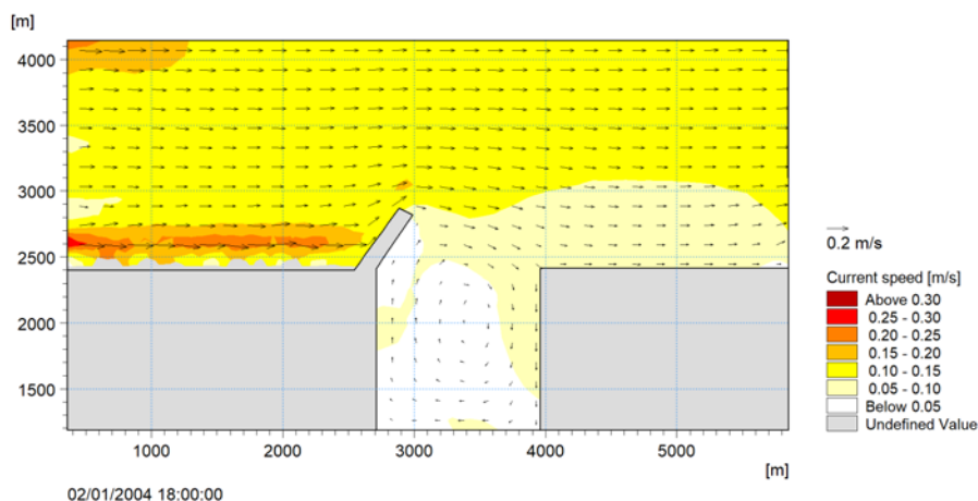
Figure 4.10 Contour and vector plot of the flow field.
