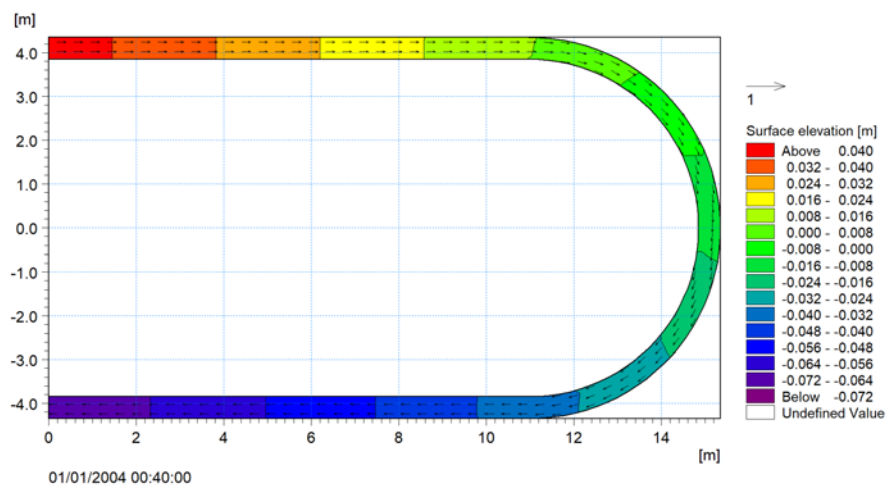
Figure 4.3 Contour plot of water surface, Vector plot of flow field.
