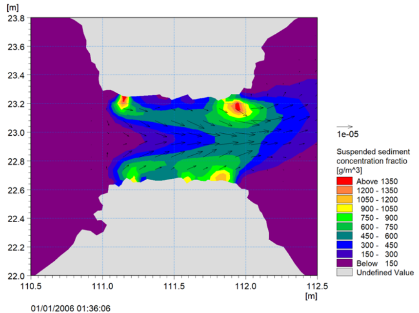
Figure 4.21 Total load transport at initial bathymetry and mid flood tide
