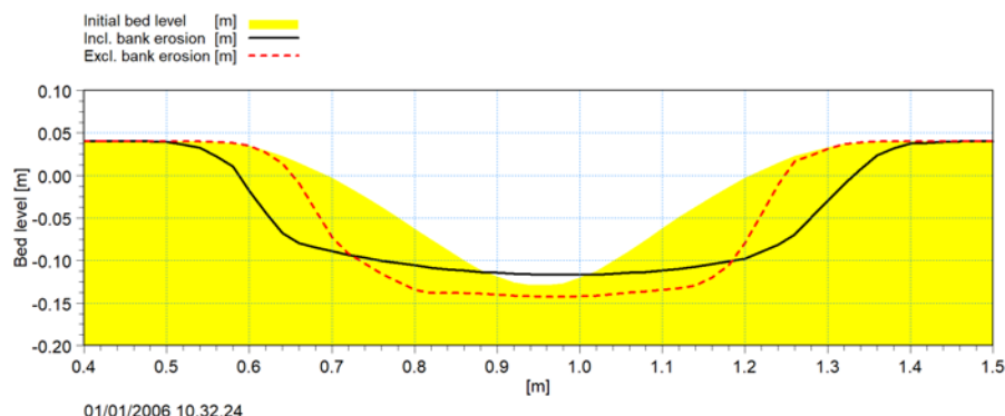
Figure 4.22 Inlet cross-section bathymetry after 5 tidal cycles. Yellow filled area: initial bathymetry Black solid line: simulated bathymetry with slope failure Red dotted line: simulated bathymetry without slope failure
