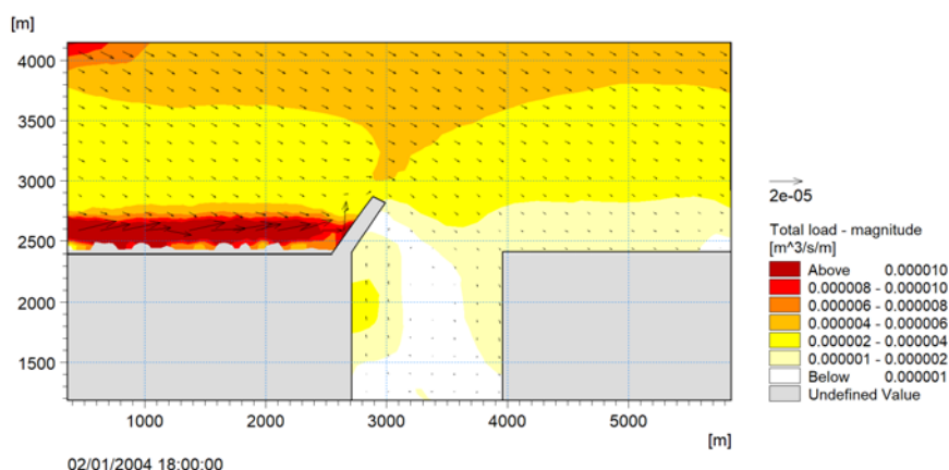
Figure 4.11 Contour and vector plot of the sand transport field.
