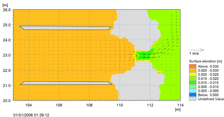
Figure 4.20 Surface elevation and current speed (magnitude and direction) at mid flood tide.
