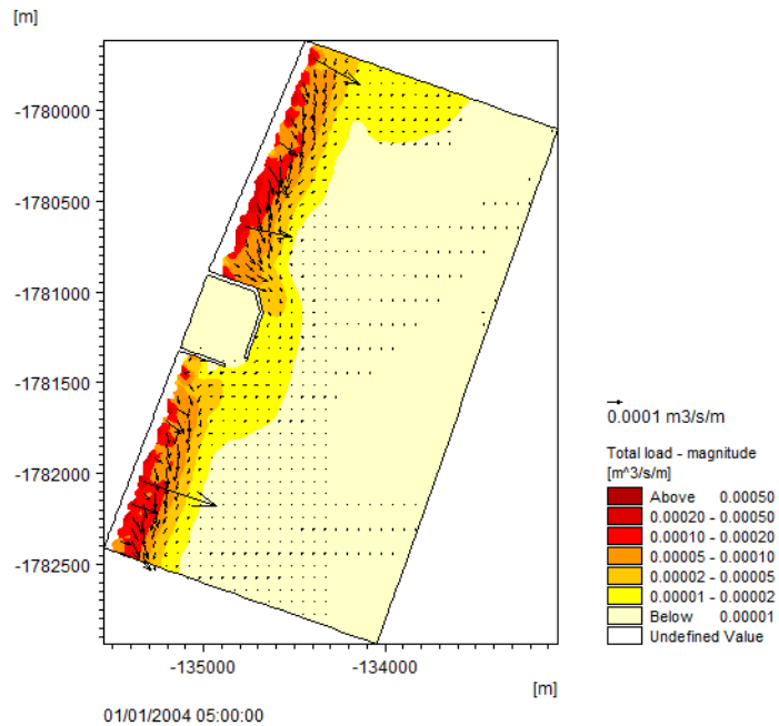
Figure 4.16 Contour and vector plot of the sand transport field.
