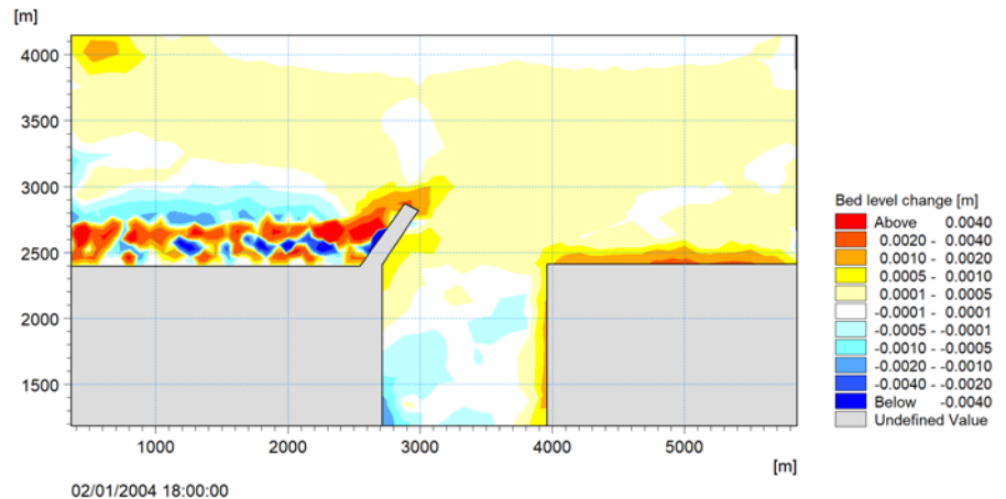
Figure 4.12 Contour plot of bed level change after 1 day.
