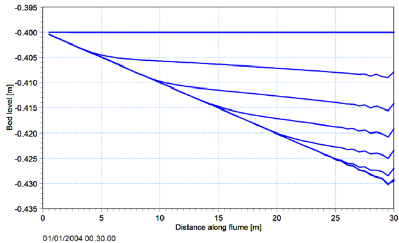
Figure 4.7 Longitudinal profile of the bed of a simulated flume every 2.5 minutes during a morphological simulation, showing the development of an equilibrium slope from an initially horizontal bed.
