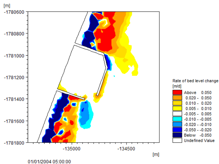
Figure 4.17 Contour plot of bed level change rate.
