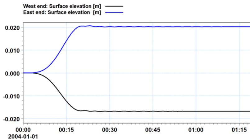
Figure 4.2 Surface elevation. Analytical estimate shows a set-up of 0.039 m.
