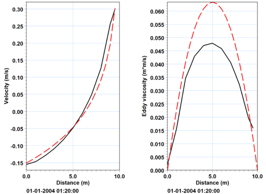
Figure 4.3 Vertical velocity profile and eddy-viscosity profile. Full line: calculated values.
