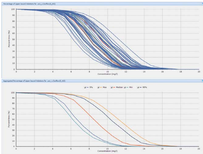
Figure 13.3 Results of the Uncertainty Analysis experiment: Percentage of Upper Bound Violation for Nitrate concentration in the effluent, all runs (top) and aggregated values (bottom)
