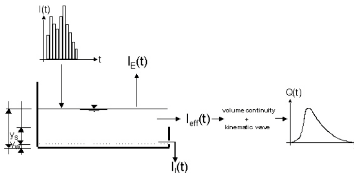
Figure 3.1 The simulated processes in the Surface runoff model B.
