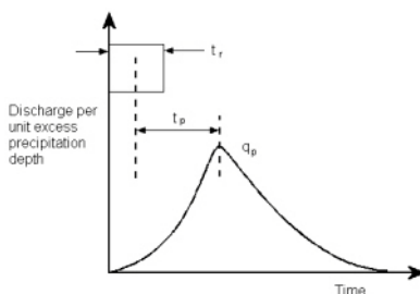
Figure 5.4 Snyder's Synthetic Unit Hydrograph
