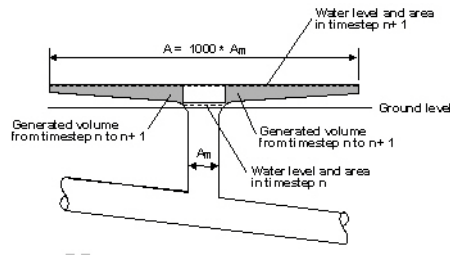
Fig A.4.9 Simulation of surface flooding
