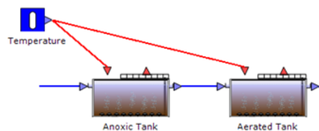
Figure 8.15 The Temperature data input Block controlling the manipulated interface variable “Temperature” of the two activated sludge tanks
