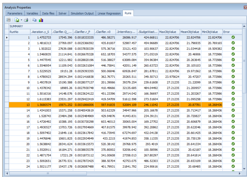
Figure 10.4 Runs tab page and best run for the Global Sensitivity Analysis experiment
