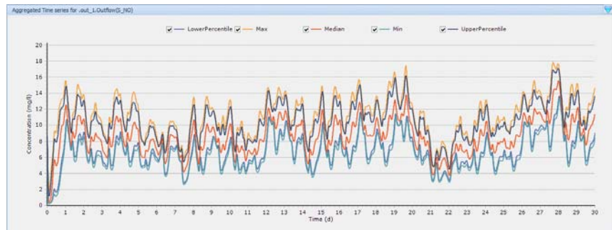
Figure 13.5 Aggregated Time series Criteria for Nitrate concentration in the effluent
