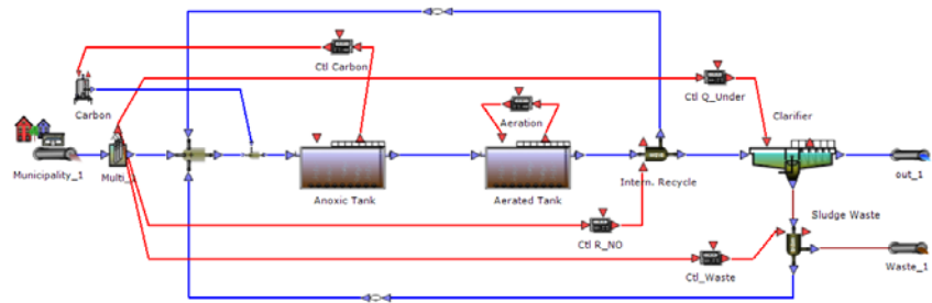
Figure 11.6 Final layout for the TwoASU_PE case
