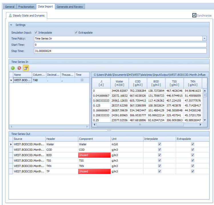
Figure 7.9 Import data (custom dataset) for the characterisation of the ASM1 influent
