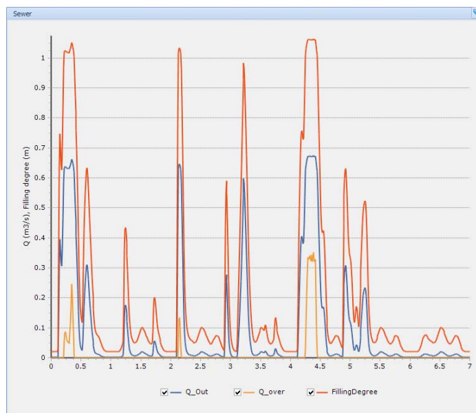
Figure 15.3 Flow rate and filling degree in the sewer
