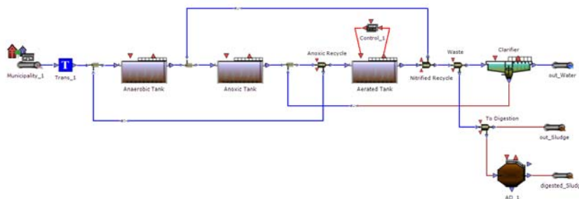
Figure 14.2 Final layout for the PWM_SA experiment
