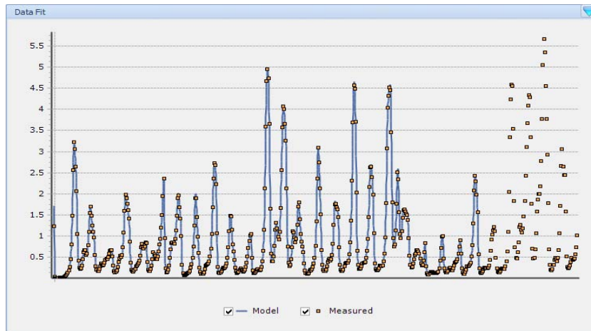
Figure 11.2 Data fit: measured data point vs. simulated values for nitrate concentration in the Anoxic tank
