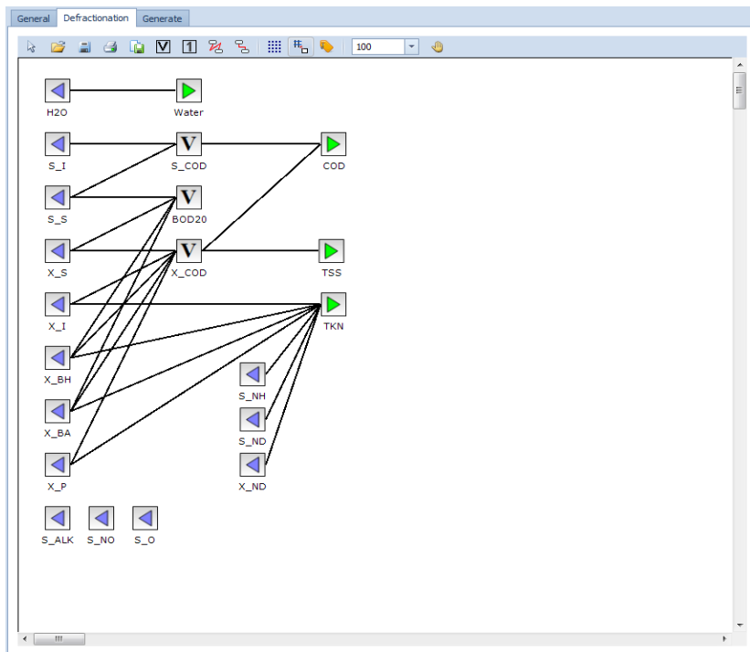
Figure 7.12 Default ASM1 De-fractionation Model
