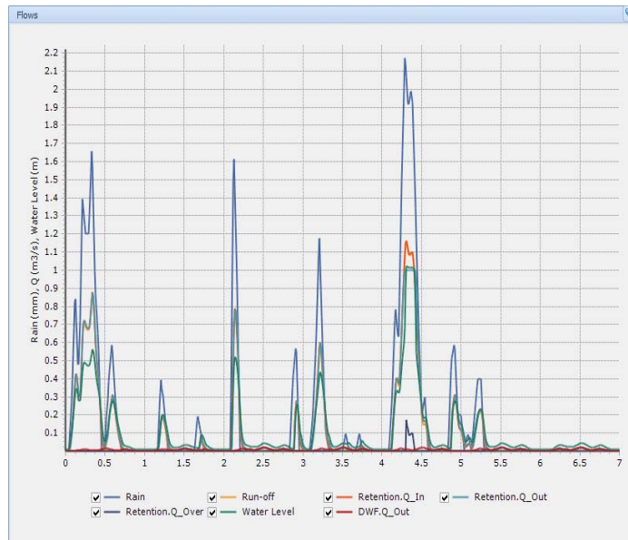
Figure 15.2 Rainfall and flow rate in the catchment
