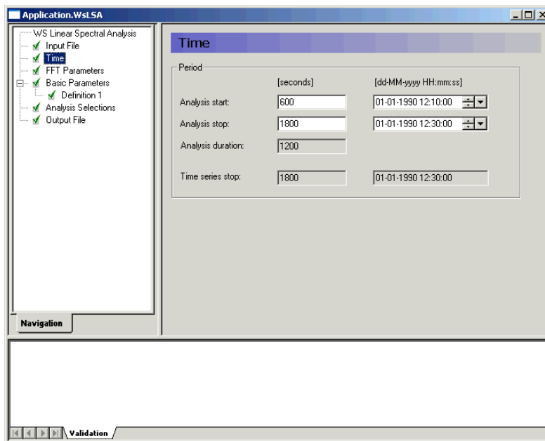
Figure 3.3 Time dialog
