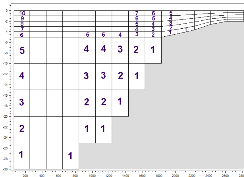
Figure 24.1 Example of layer numbers in point output specification in case of combined sigma-z level mesh
