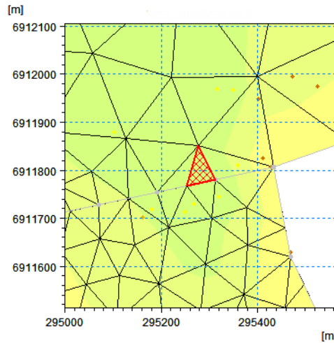
Figure 15.29 Marked grid cell for smallest restrictive time step when calculation is based on the water level.
