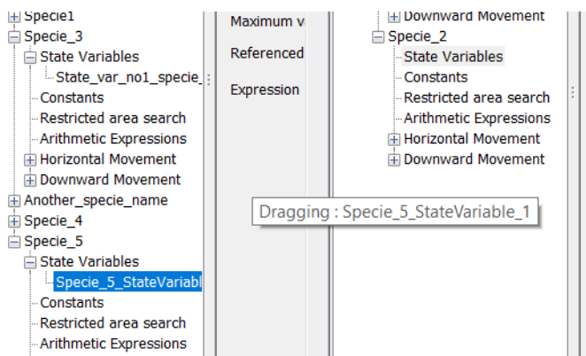
Figure 3.17 Dragging item to another template
