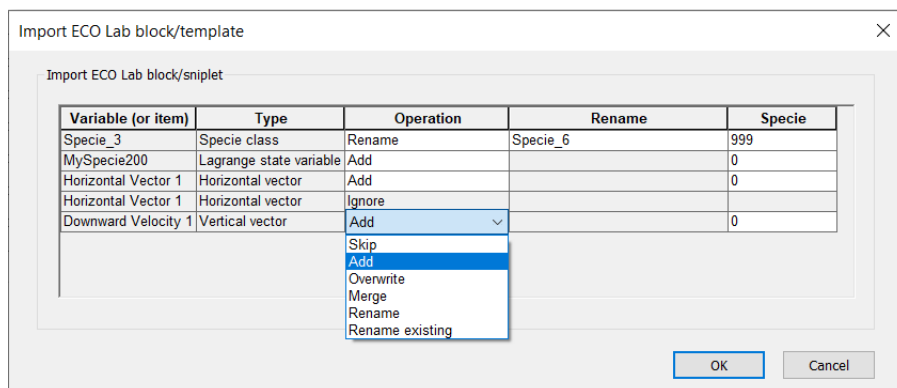
Figure 3.9 Import 'snippet' dialog
