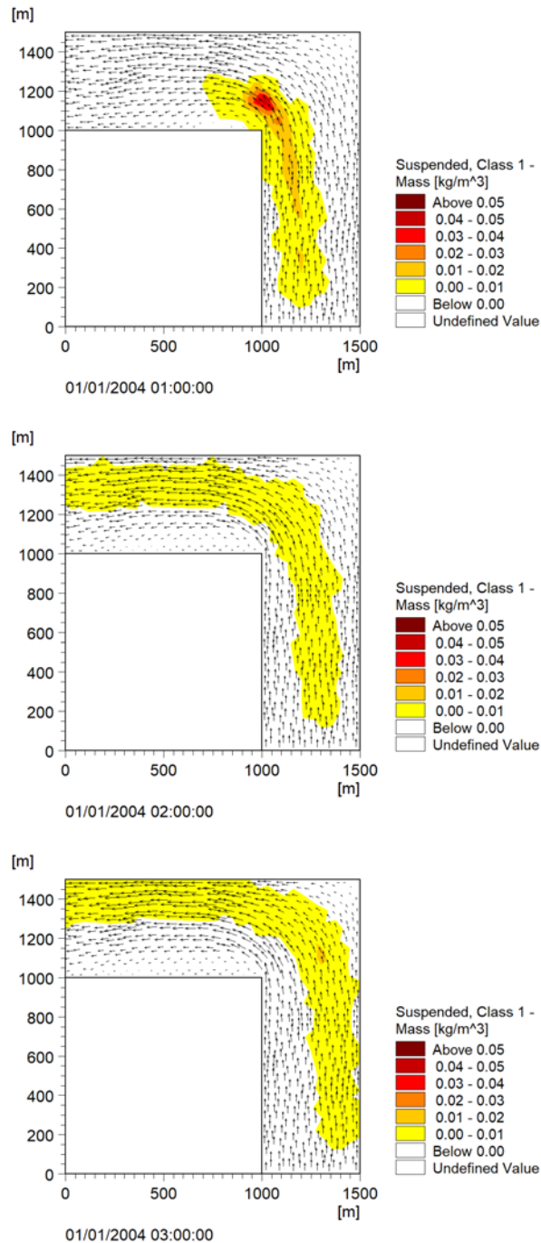
Figure 4.5 Concentration of suspended material (arrows indicate currents) Upper: after 1 hour Middle: after 2 hours Lower: after 3 hours
