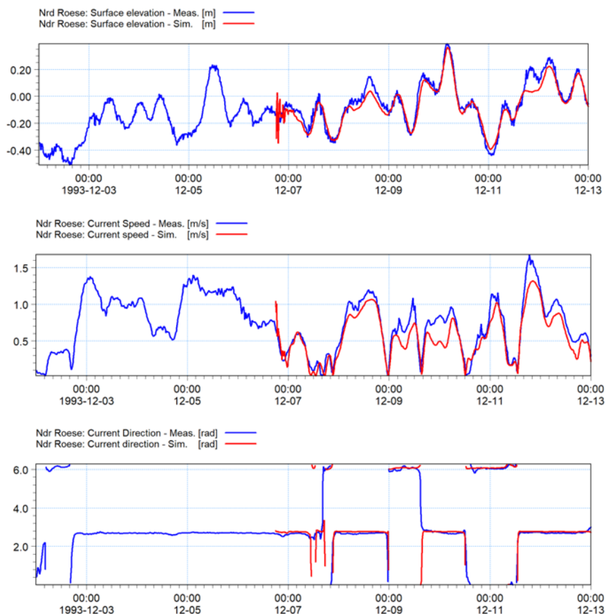
Figure 4.12 Measured values versus simulated values at Ndr. Roese Upper: Water level Middle: Current speed Lower: Current direction
