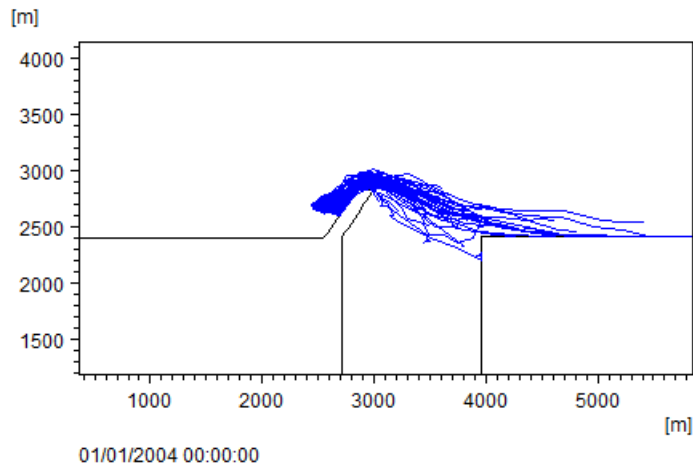
Figure 4.8 Float tracks for particle class “Floaters”
