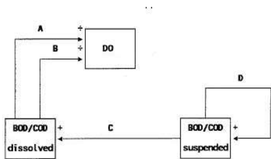
Figure 2.1 Conceptual diagram of the BOD/COD-DO model. Process A is de-gradation in biofilm, process B is degradation in water phase, process C is hydrolysis and process D is growth of heterotrophics
