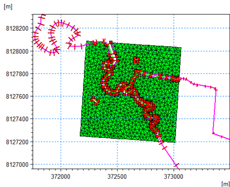
Figure 2.6 Close up of the combined river and flood plain model
