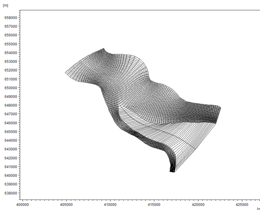
Figure 2.10 The final grid - Gorai-grid.dfs2
