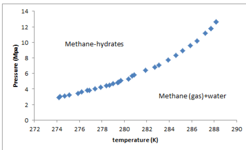
Figure C. 1 Phase system for methane ( \text{CH}_4 ) in water
