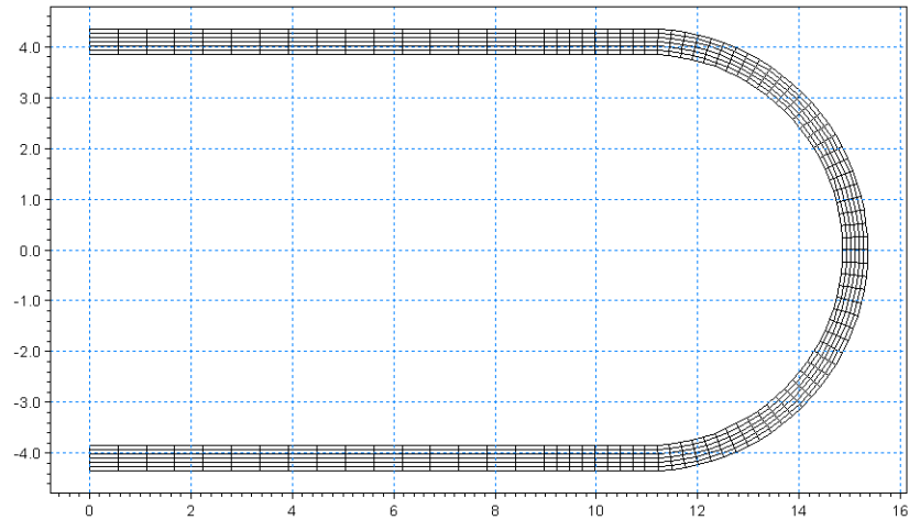
Figure 4.2 Computational mesh
