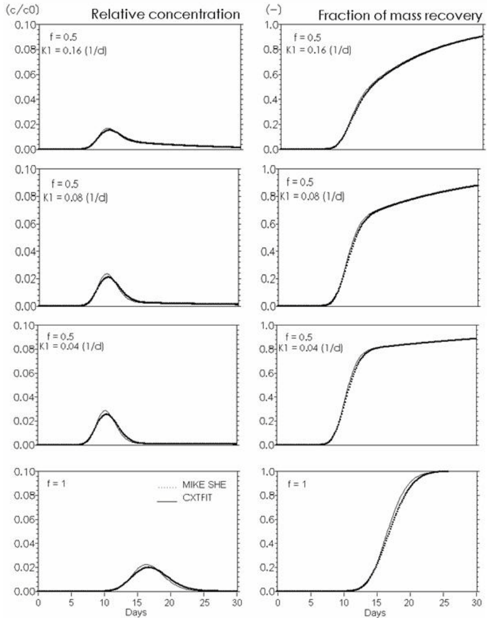
Figure 36.6 Kinetic sorption . Effects of rate constant K_1 ( d^{-1} ) in Eq.(36.9). Input to CXTFIT: f (fraction of equilibrium sorption sites). K_d = 0.5 ml/g. Input to MIKE SHE: K_d = f \cdot K_d (CXTFIT). At f=1 the function is reduced to equilibrium sorption with K_d = 0.5 ml/g.
