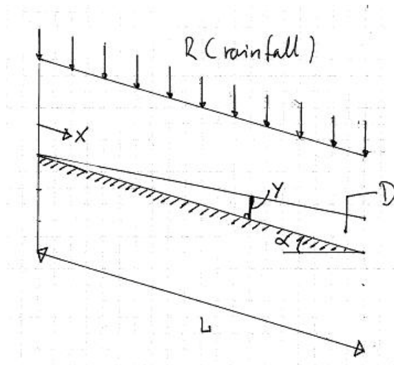
Figure 25.8 Schematic of overland flow on a plane
