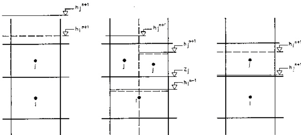
Figure 31.4 Types of vertical flow condition, a) confined conditions in nodes i and j, b) unconfined condition in node i, c) unconfined in nodes i and j, d) dry conditions in node j and confined conditions in node i.
