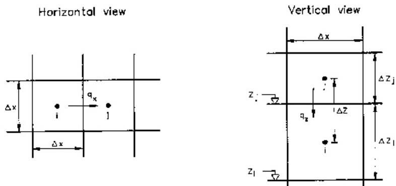
Figure 31.3 Spatial discretisation.
