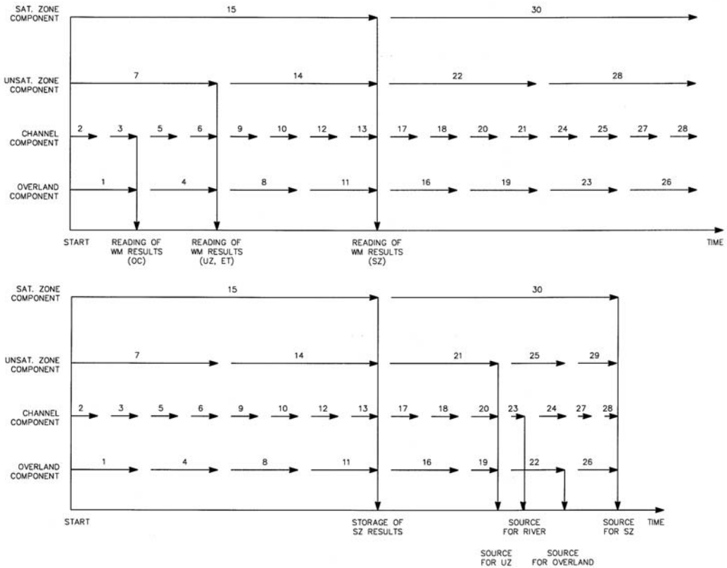
Figure 35.2 An example calculation sequence for solute transport in MIKE SHE.
