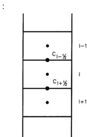
Figure 35.5 Control volume defining an internal grid.
