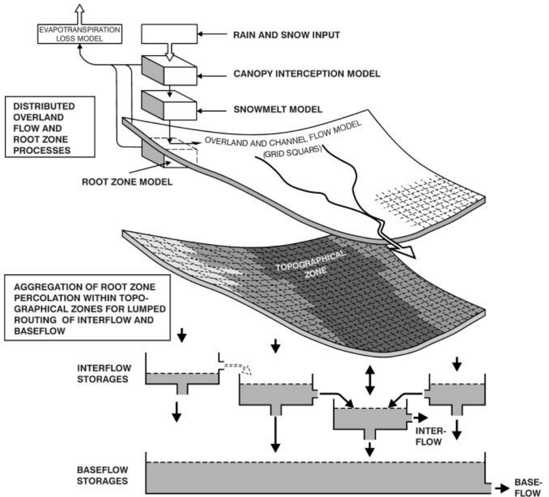
Figure 31.8 Model Structure for MIKE SHE with the linear reservoir module for the saturated zone
