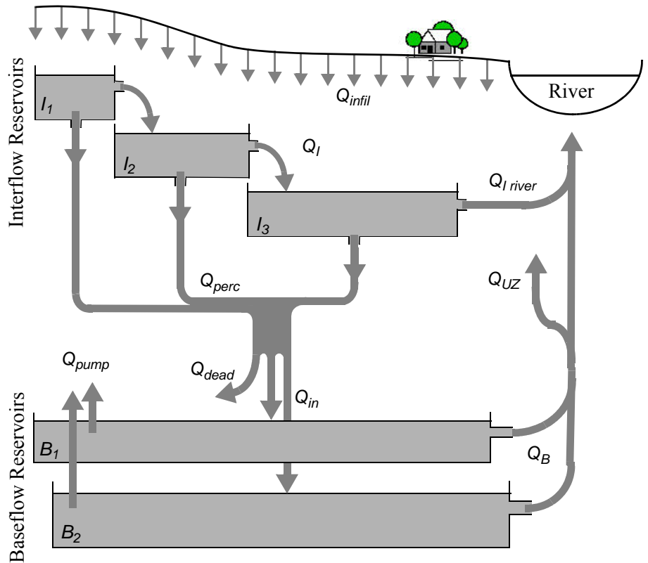
Figure 31.10 Schematic flow diagram for the Subcatchment-based, linear reservoir flow module
