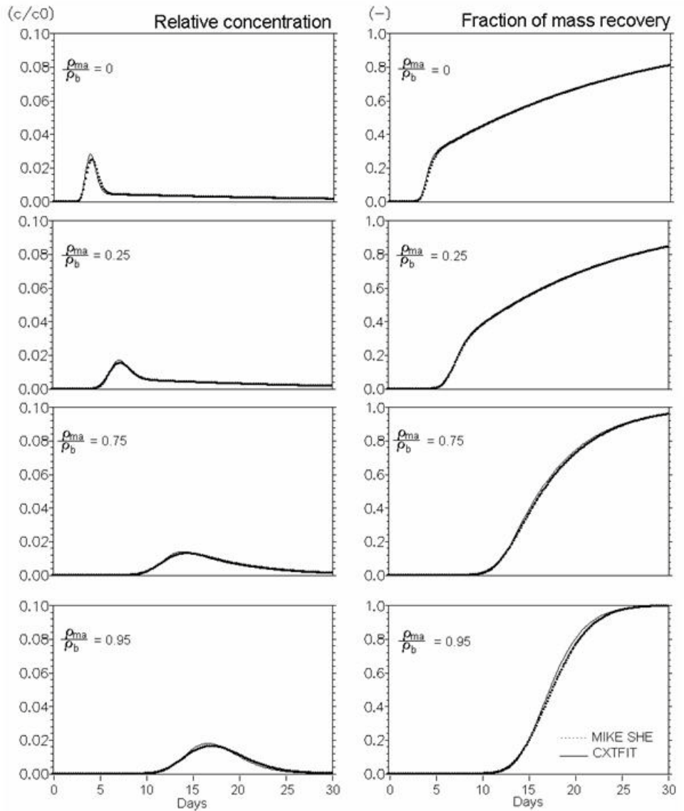
Figure 36.8 Verification of reactive solute transport in dual porosity systems. Mobile porosity = 0.25, immobile porosity = 0.05. Effect of distribution of sorption sites between mobile and immobile regions ( \rho_{ma}/\rho_b Eq. 47) ( K_d = 0.5 ml/g, mass transfer coefficient ( \beta_s ) = 0.08 d -1 ).
