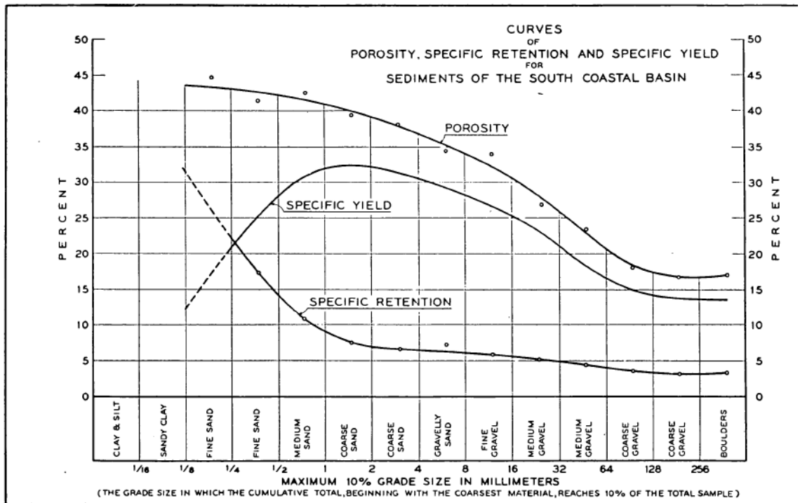
Figure 30.1 Relation between Specific Yield, Porosity and Field Capacity (from USGS OFR 63-59, Figure 3)
