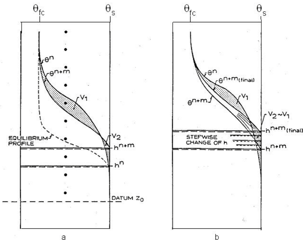
Figure 29.4 a) Soil moisture content at two times n and n+m without corrections, and b) Soil moisture content at time n+m before and after correction.
