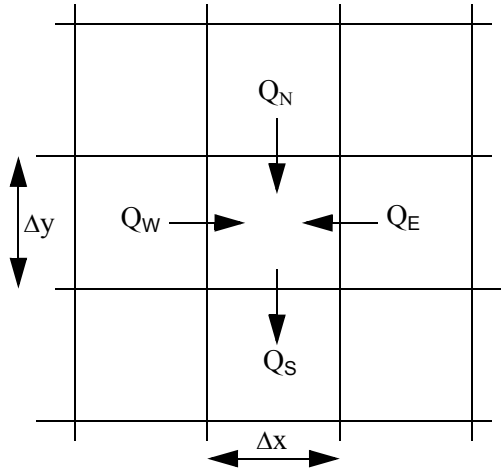
Figure 25.1 Square Grid System in a small Region of a MIKE SHE model
