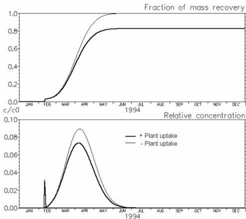
Figure 36.11 Illustration of the effect of plant uptake on solute breakthrough. Plant uptake was simulated with f_c = 0.5 . The early peak concentrations arise from macro pore transport and were almost alike in the two simulations.
