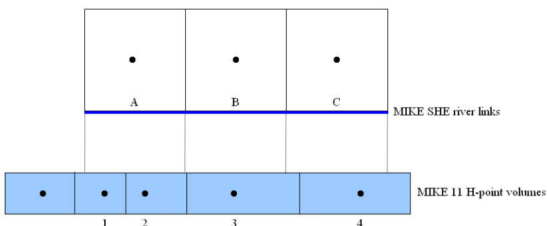
Figure 28.3 Sharing of MIKE Hydro River H-point volumes with MIKE SHE river links
