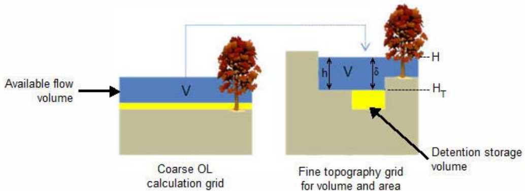
Figure 26.1 The constant volume from the coarse grid is transferred to the fine scale grid
