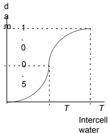
Figure 25.3 Default damping function for numerical stability at low gradients
