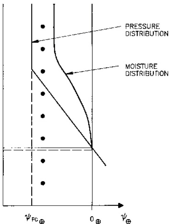
Figure 29.2 Illustration of initial soil moisture profile and pressure head profile.
