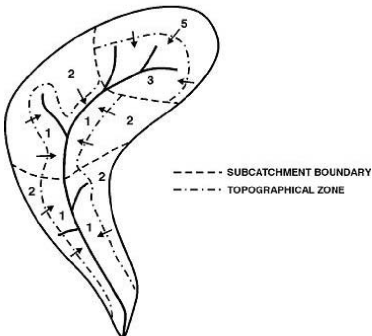
Figure 31.9 Example of Desegregation of a Catchment into Sub-catchments and Topographical Zones
