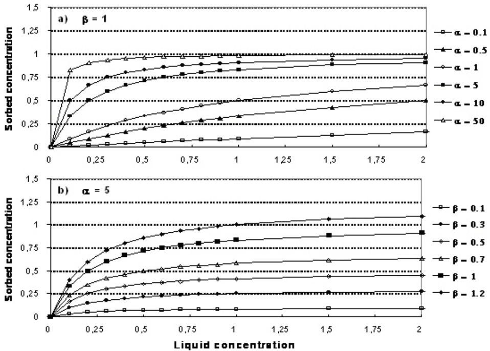
Figure 36.2 Illustration of the Langmuir isotherm. a) effect of change in \alpha , b) effect of change in \beta .
