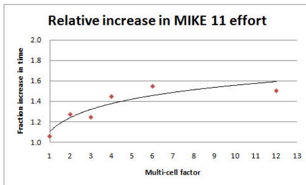
Figure 26.8 Increase in MIKE Hydro River run time as a function of multi-cell factor.
