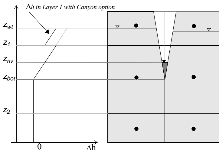
Figure 31.6 Water table elevation versus the head difference.
