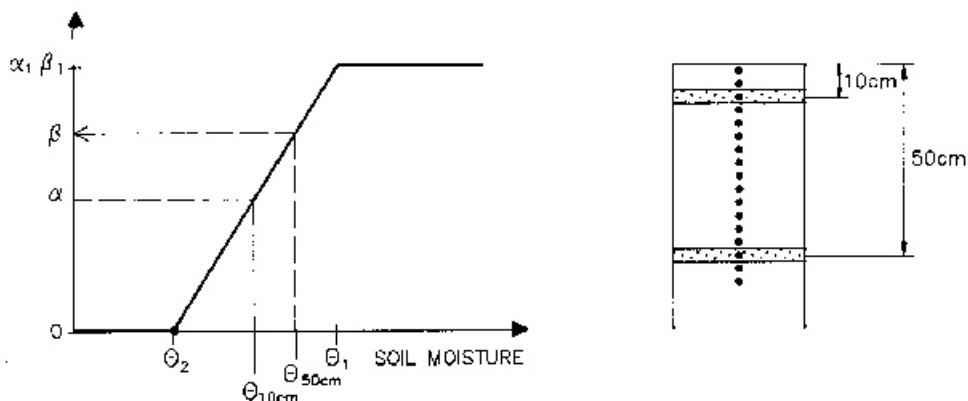
Figure 29.3 \alpha and \beta as a function of the soil moisture content 10 cm and 50 cm below the ground surface, respectively.
