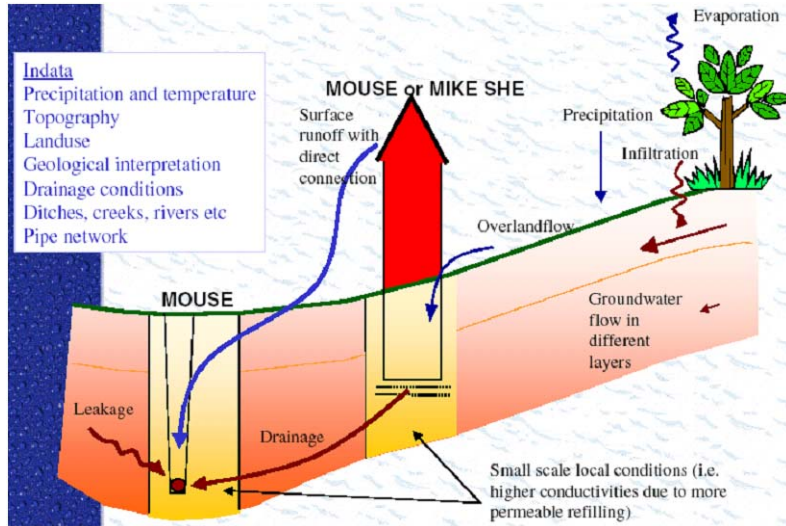
Figure 33.1 MIKE SHE to MIKE URBAN coupling linkages
