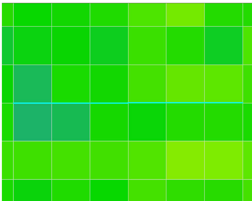
Figure 26.6 Interpolation of the 5-foot LIDAR data to the 1500ft model grid
