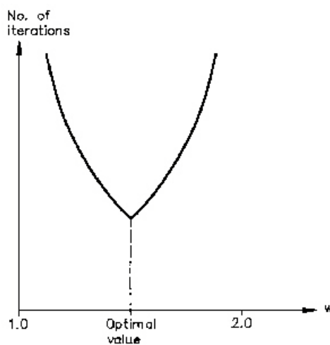
Figure 31.5 Empirically relationship between the relaxation coefficient w and number of iterations for a given model.
