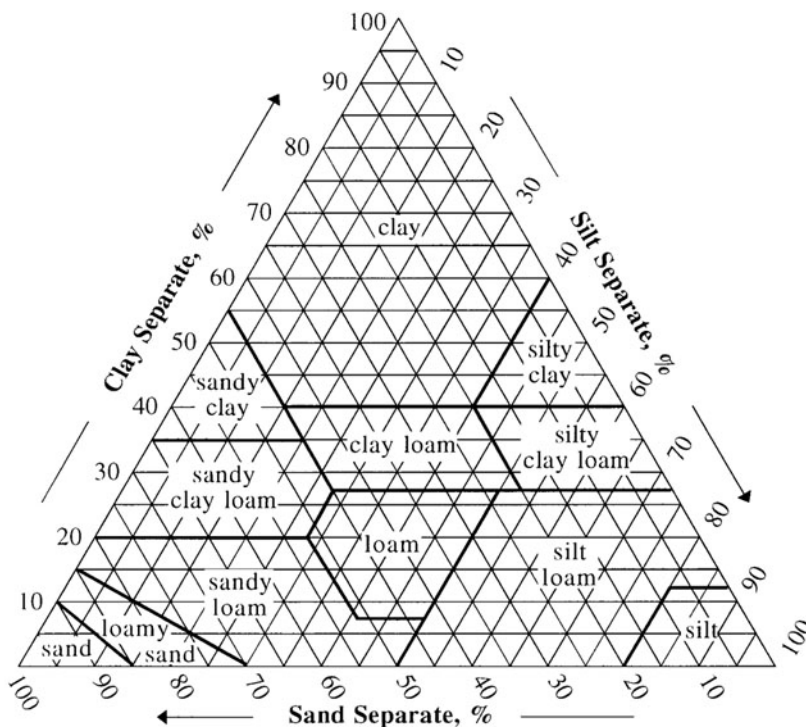
Figure 30.2 USDA Soil texture classification by grain size distribution
