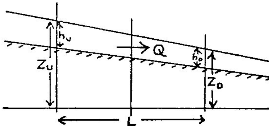
Figure 25.2 Overland flow across grid square boundary.
