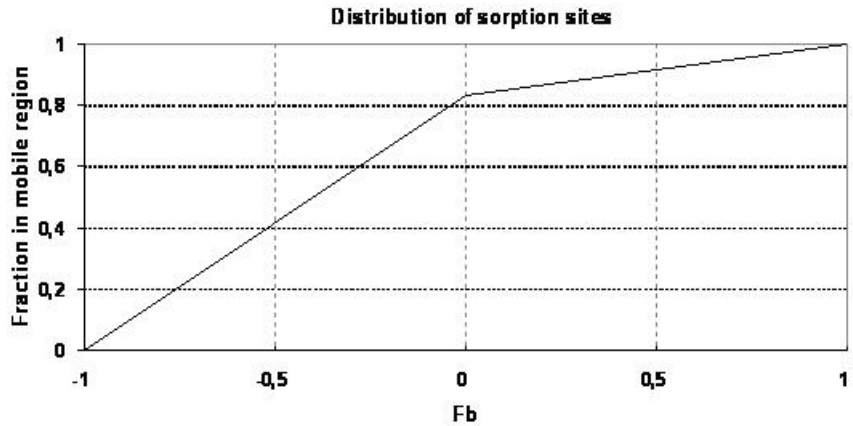
Figure 36.3 Illustration of the fraction of sorption sites located in the macro pore region ( \rho_{ma}/\rho_b ) as a function of F_b . Mobile porosity = 0.25, immobile porosity=0.05.
