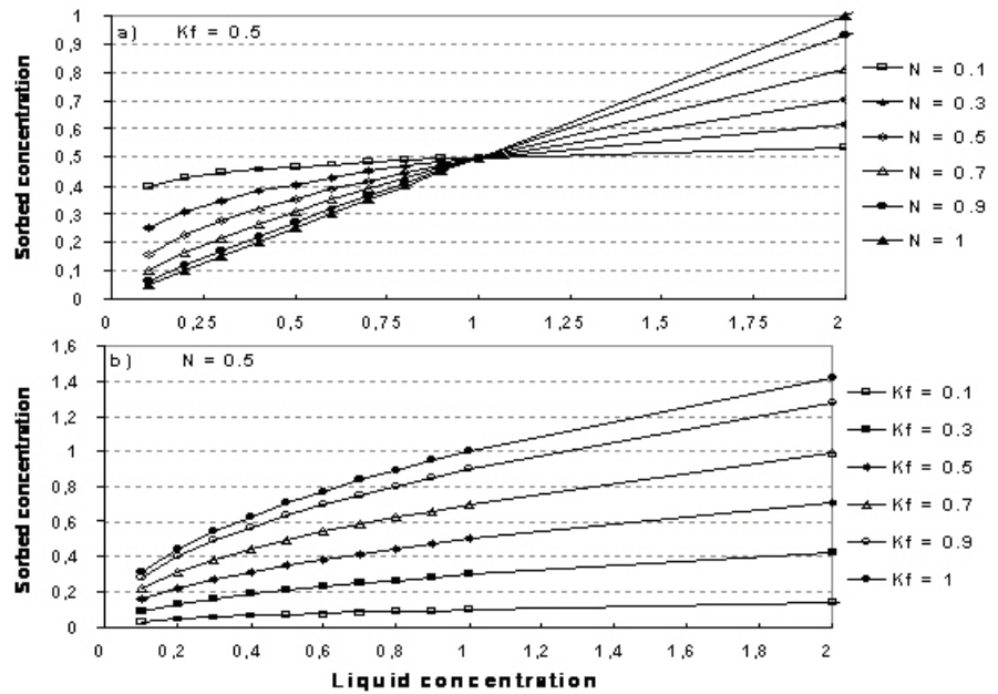
Figure 36.1 Illustration of the Freundlich isotherm. a) effect of change in N, b) effect of change in Kf
