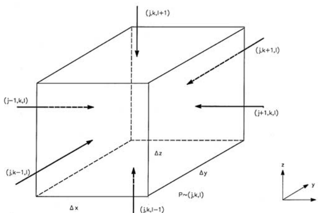
Figure 35.3 Control volume defining an internal SZ grid.
