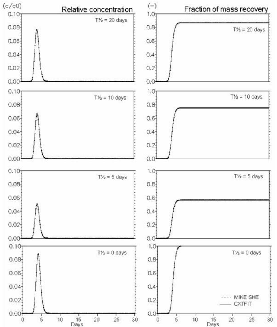
Figure 36.10 Verification of the description of first order degradation. Effect of half life time - T_{1/2} ( \Lambda ) (days) (Eq. (36.12)).
