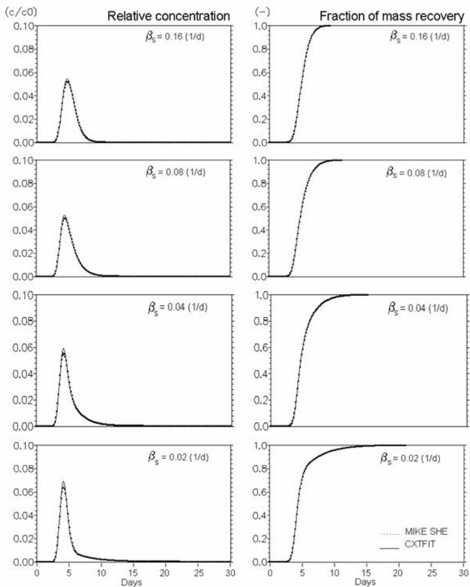
Figure 36.7 Conservative solute transport in dual porosity systems. Mobile porosity = 0.25, immobile porosity = 0.05. Effect of mass transfer coefficient ( \beta_s in Eq. (35.16) ( d^{-1} )).
