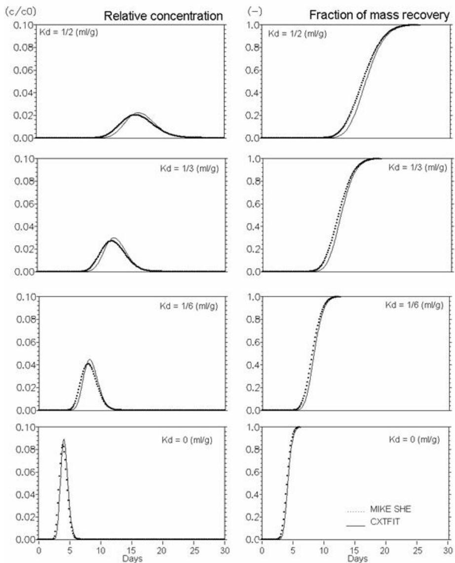
Figure 36.5 Linear equilibrium sorption. Effect of K_d (ml/g)
