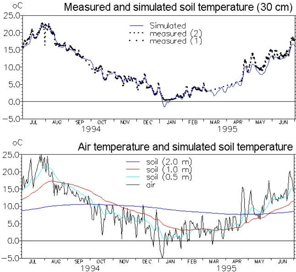
Figure 36.4 Application of the soil temperature function. Top: measured and simulated soil temperature in 30 cm depth (measurements were based on two replicates). Bottom: soil temperatures simulated in different depths based on measured air temperatures.
