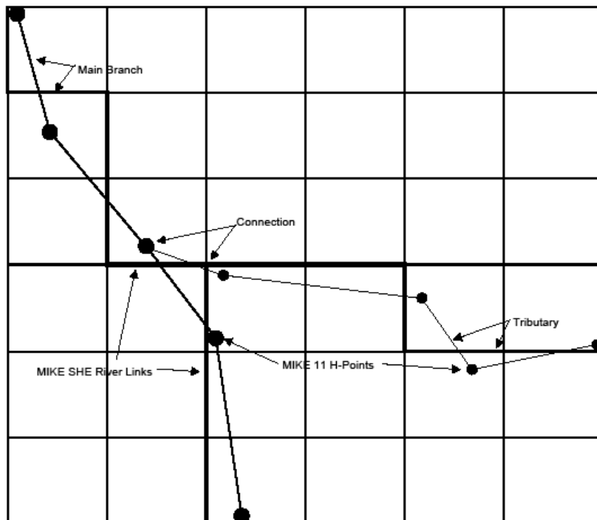
Figure 28.1 MIKE Hydro River Branches and h-points in a MIKE SHE Grid with River Links
