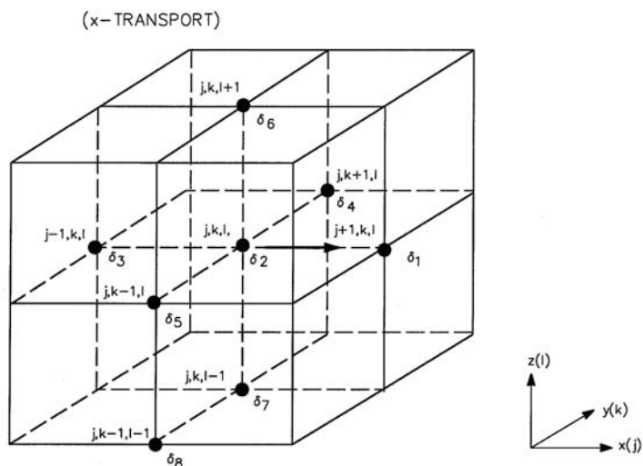
Figure 35.4 Location of interpolation weights for determination of concentrations at the location (j+1/2, k, l) - a grid boundary.
