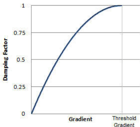
Figure 25.5 Alternative damping function activated by an Extra Parameter.
