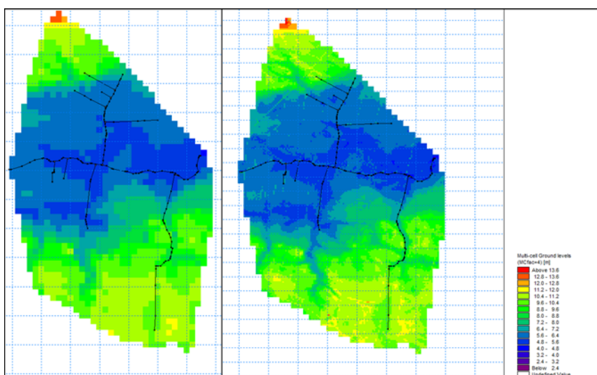
Figure 26.9 Example of preprocessed data - topography using a 100 meter resolution and a sub-scale factor of 4 (25 m sub-scale resolution)
