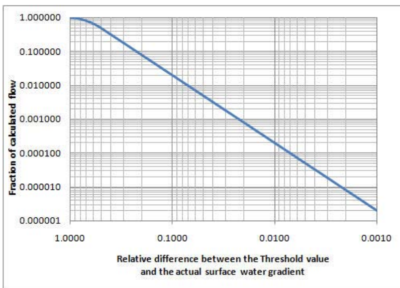
Figure 25.4 Actual overland flow as a function of the difference between the threshold gradient and the surface water gradient based on Equations (25.19) and (25.20).
