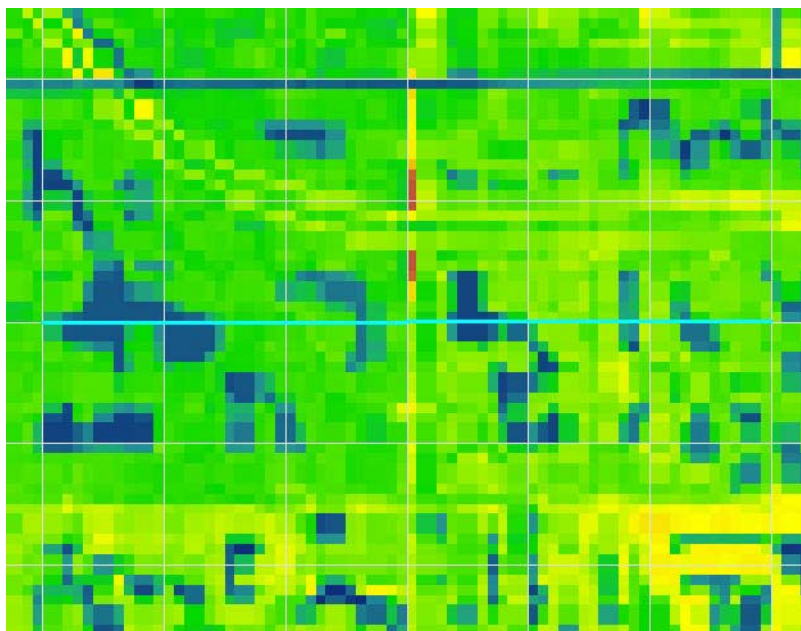
Figure 26.5 Interpolation of the 5-foot LIDAR data to the 125ft model grid
