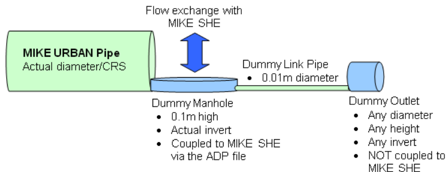
Figure 33.2 Work around for discharging MIKE URBAN outlets to MIKE SHE
