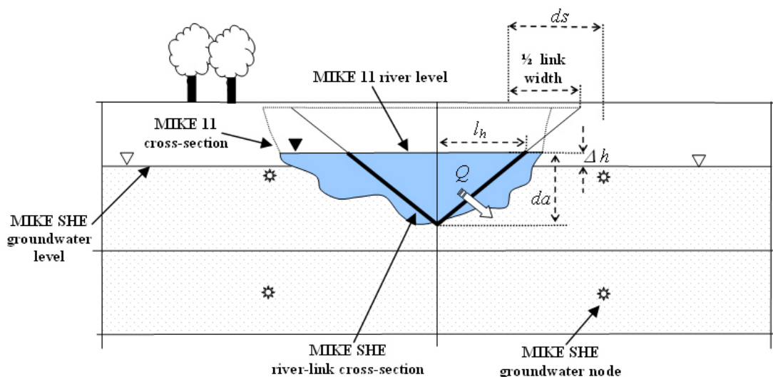
Figure 28.2 A typical simplified MIKE SHE river link cross-section compared to the equivalent MIKE Hydro River cross-section
