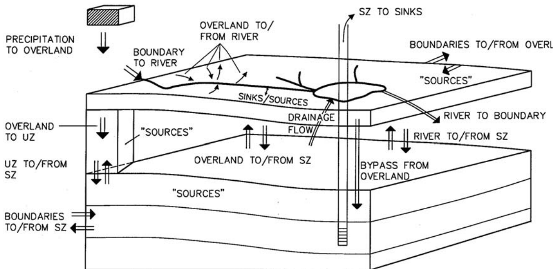
Figure 35.1 Outline of the different transport possibilities between components and boundaries.
