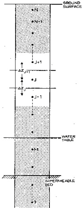
Figure 29.1 Vertical Discretisation in the Unsaturated Zone.
