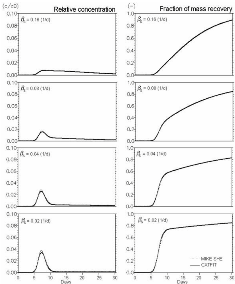
Figure 36.9 Verification of reactive solute transport in dual porosity systems. Mobile porosity = 0.25, immobile porosity = 0.05. Effect of mass transfer coefficient ( \beta_s in Eq. (35.16) ( \text{d}^{-1} )). K_d = 0.5 \text{ ml/g} , \rho_{ma}/\rho_b = 0.25 (Eq. (36.10)).
