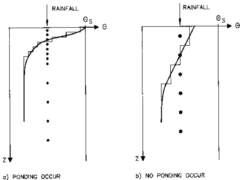
Figure 30.3 Examples of different increments in the soil profile and the resulting water content distribution of 1-3 cm for detailed studies and 3-5 cm for catchment studies. Further down in the profile larger increments can be chosen ranging from 10 cm to 30 cm.
