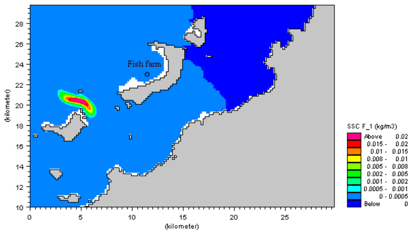
Figure 3.8 Maximum suspended sediment concentration site 1
