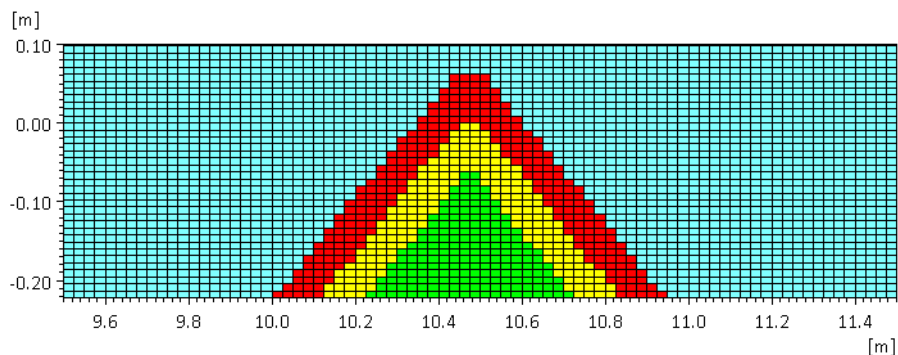
Figure 4.14 3D porosity map (dfsu-file) with three different porous zones. Yellow: Core; Green: filter layer; Red: armour. layer
