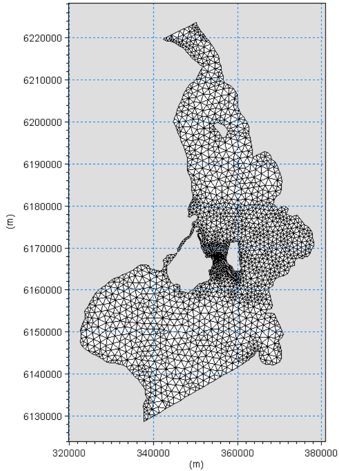
Figure 4.11 Computational mesh
