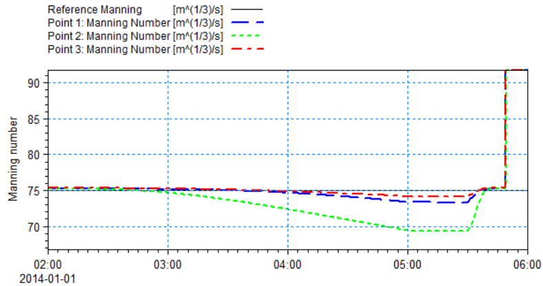
Figure 3.22 Time series of simulated Manning numbers during simulation. Values derived from Point 1, 2 and 3 (see Figure 3.17). Reference Manning of 75 m 1/3 /s is shown for comparison
