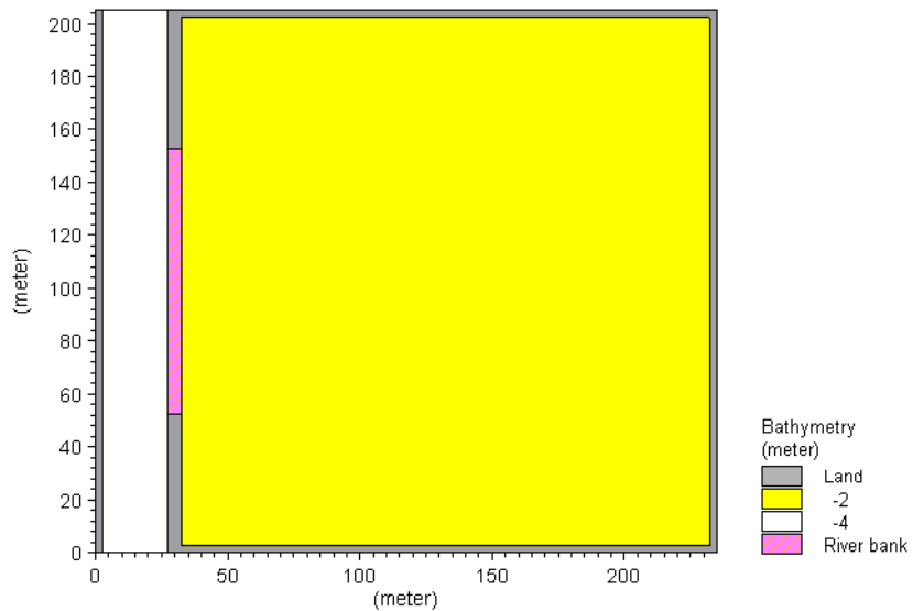
Figure 3.7 Filling of a retention basin, model layout. \Delta X=5\text{m}
