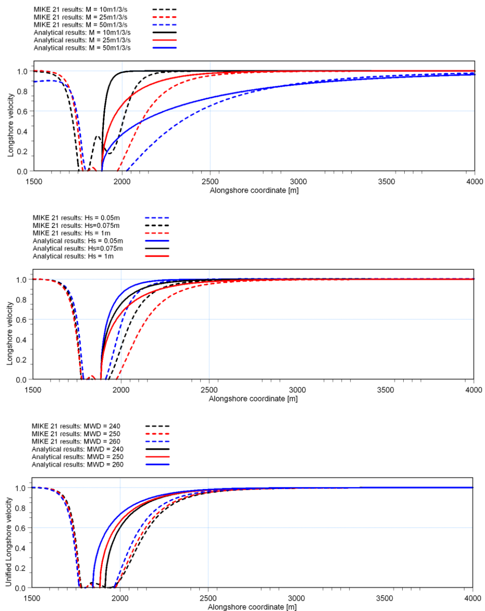
Figure 5.5 Non-dimensional longshore velocity at break line vs. longshore coordinate. Upper : MWD=250 deg.N and H s =1 m; Middle: MWD=250 deg.N and M=25 m 1/3 /s; and Lower: M=25 m 1/3 /s and H s =1 m.
