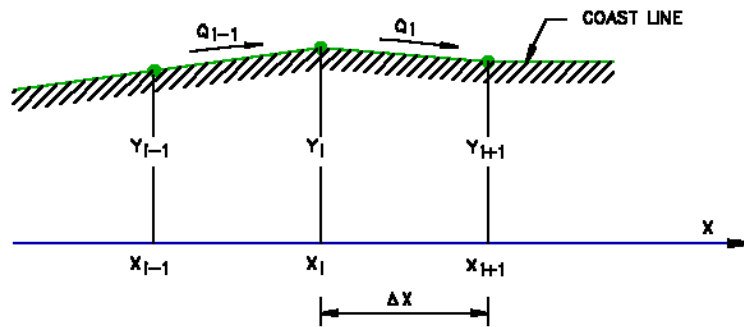
Figure 5.21 Longshore discretization
