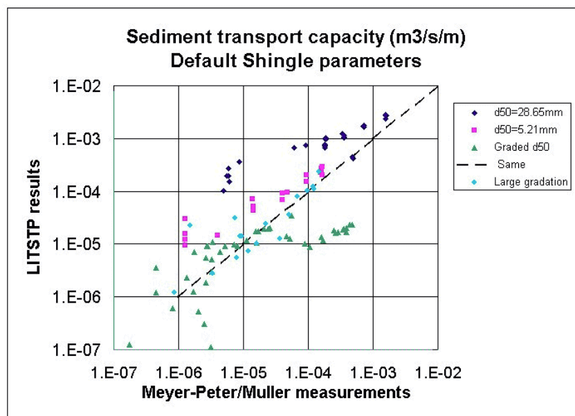
Figure 2.12 Comparison between LITPACK results and measurements of Meyer-Peter & Müller (1948). Default friction coefficients: \mu_{td} = 0.5 , \mu_{ts} = 1.0 .
