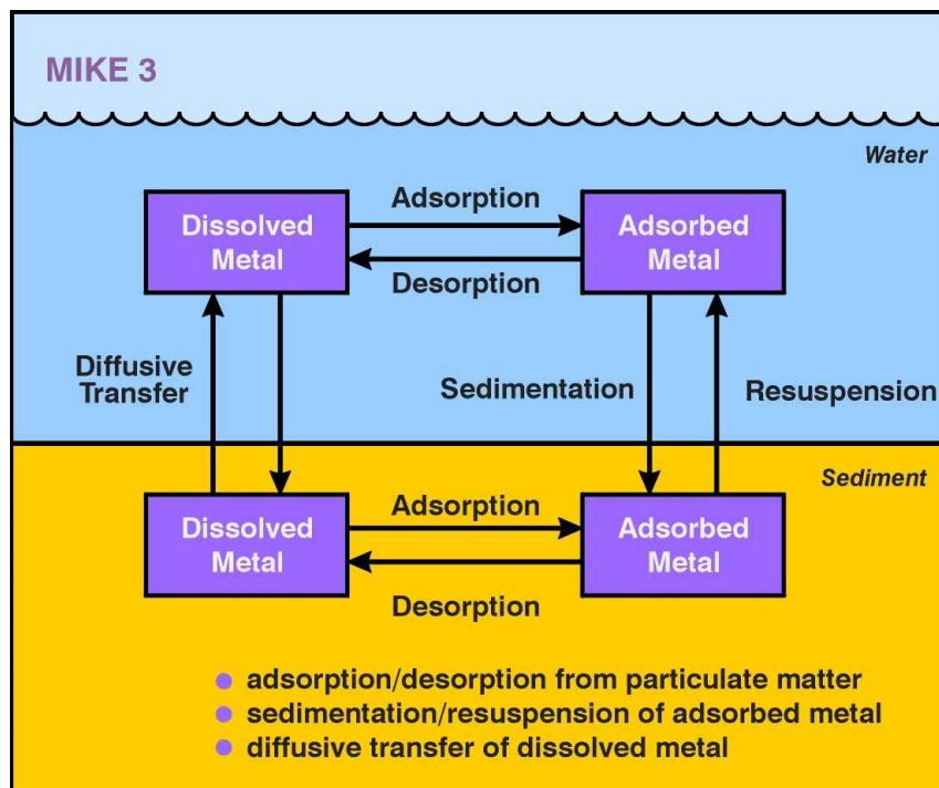
Figure 2.1 Sketch showing the transfer processes included in the Heavy Metal template
