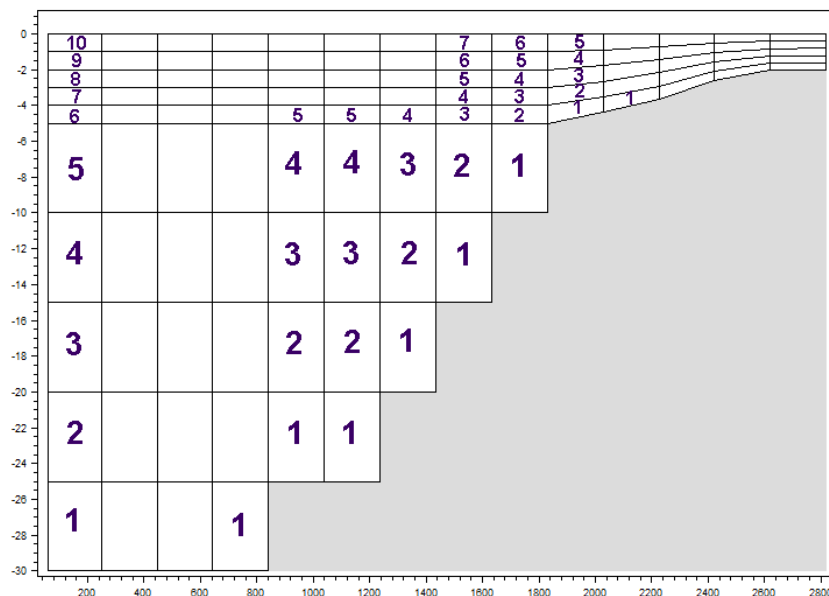
Figure 5.7 Example of layer numbers in point output specification in case of combined sigma-z level mesh.
