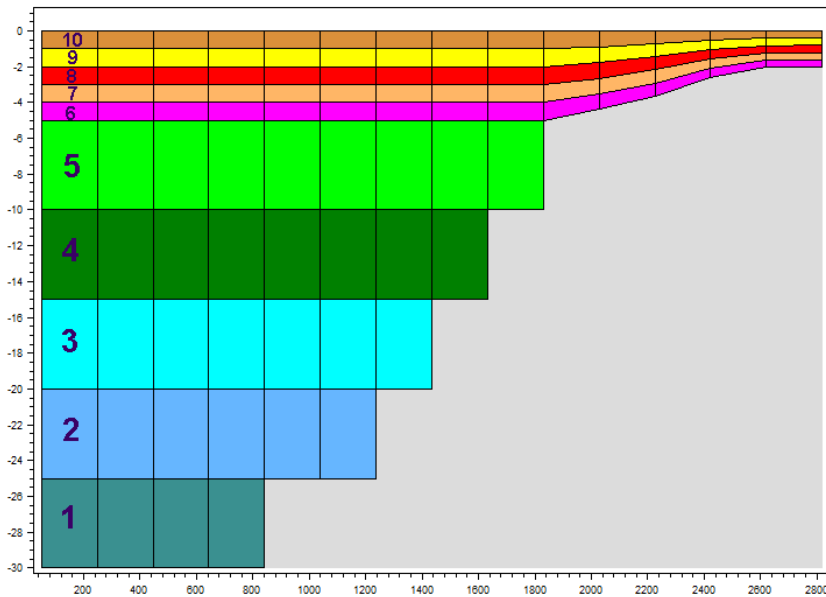
Figure 6.24 Example of layer numbers in volume output specification in case of combined sigma-z level mesh.
