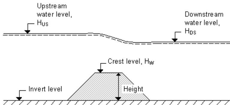
Figure 6.6 Definition sketch for Weir Flow
