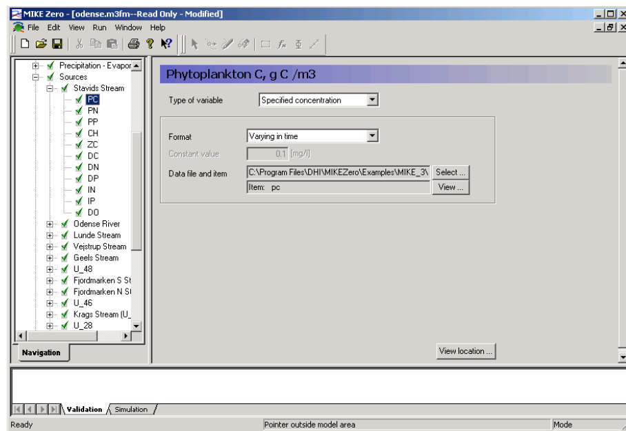
Figure 4.35 MIKE 3 Flow Model FM: Specifying concentrations for the advective MIKE ECO Lab state variables in Stavsids Stream
