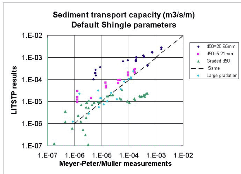
Figure 2.12 Comparison between LITPACK results and measurements of Meyer-Peter & Müller (1948). Default friction coefficients: \mu_d = 0.5 , \mu_s = 1.0 .
