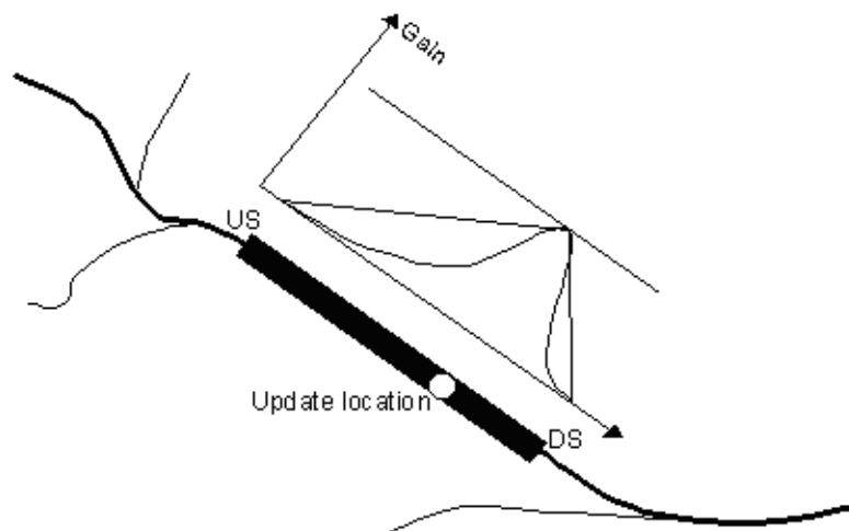
Figure 8.1 Definition of gain function for a measurement (update) location. Note that updates cannot take place across river junctions
