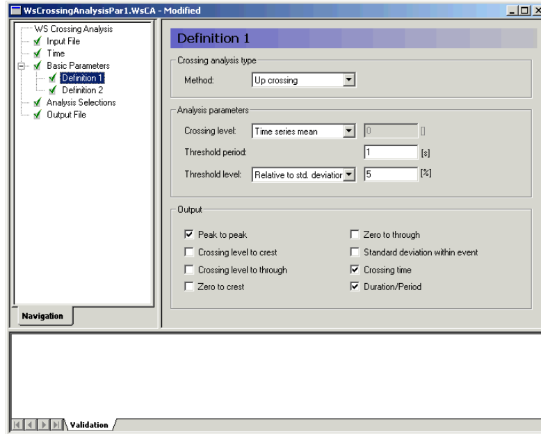
Figure 6.5 Definition dialog
