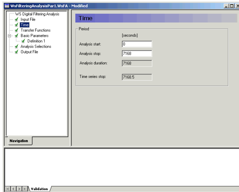
Figure 4.4 Time dialog
