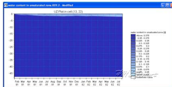
Figure 26.37 Example UZ plot of unsaturated zone water content
