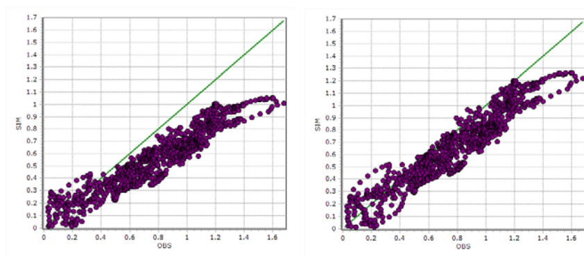
Figure 25.5 Scatter plot OBS vs SIM for the current speed parameter at NR Left: Run1, Right: Run2
