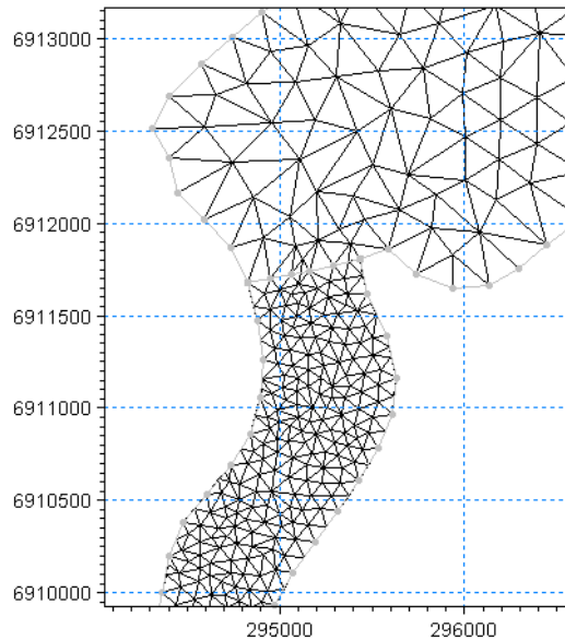
Figure 15.24 Triangulation using two zones with different maximum element areas
