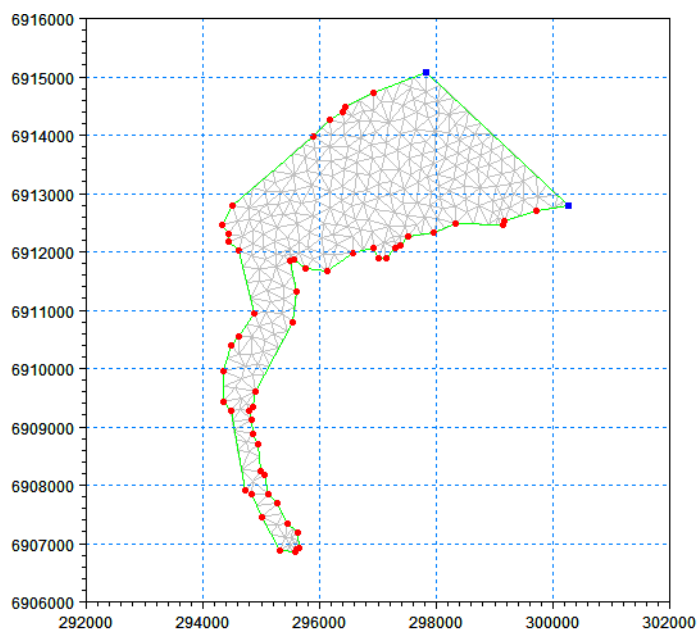
Figure 15.13 Generated mesh
