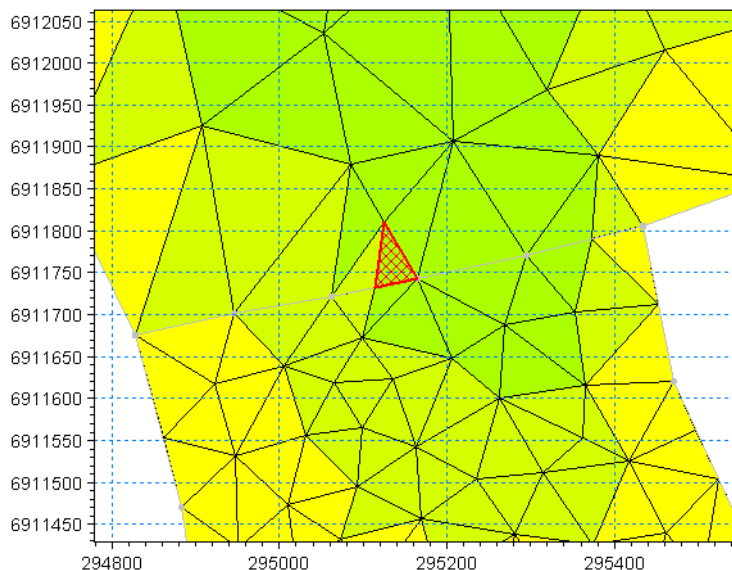
Figure 15.29 Marked grid cell for smallest restrictive time step when calculation is based on the water level.
