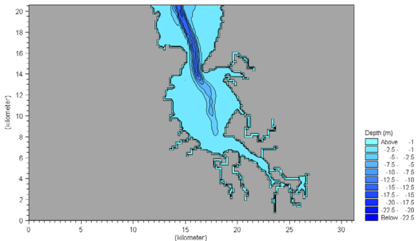
Figure 3.12 Bathymetry
