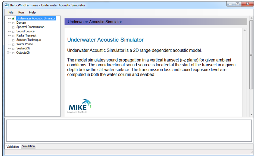
Figure 4.1 UAS Editor
