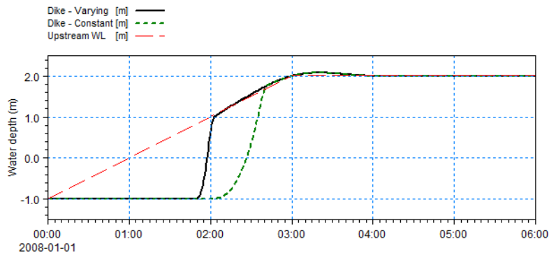
Figure 3.15 Resulting water level using during dike with time-varying crest level Black solid line: water level at position (100m, 100m) during failure. Green dashed line: water level for constant crest level. Red dashed line: upstream water level in river for reference
