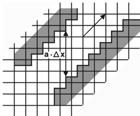
Figure 6.6 Flow in a channel at 45 degrees
