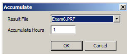
Figure 10.10 Accumulate dialog
