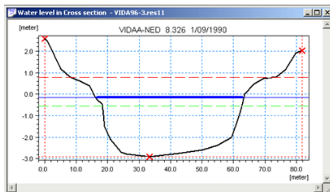
Figure 13.17 Typical Cross Section Plot
