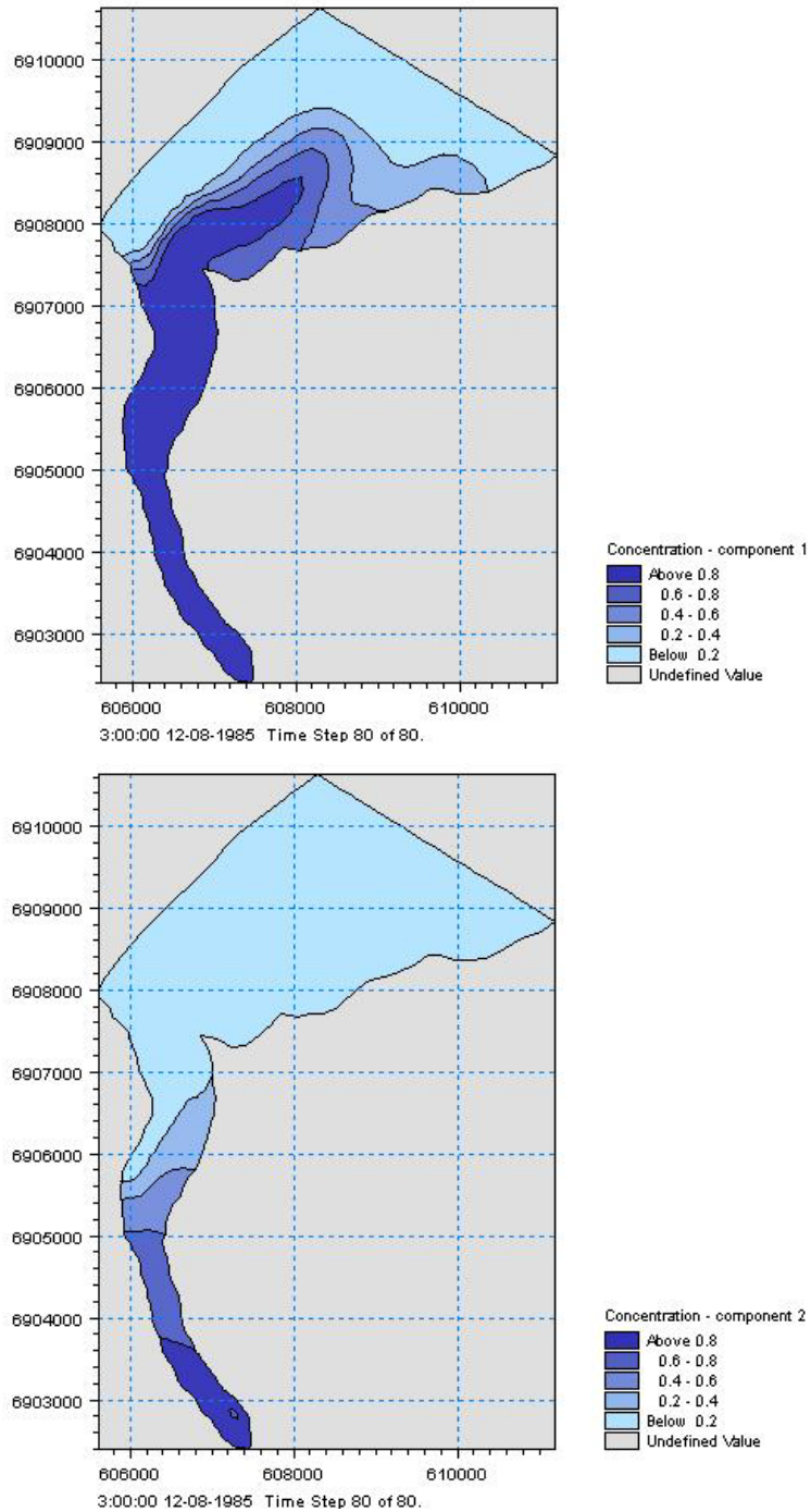
Figure 4.3 Contour plot of the concentration for the conservative component (top) and the decaying component (bottom).
