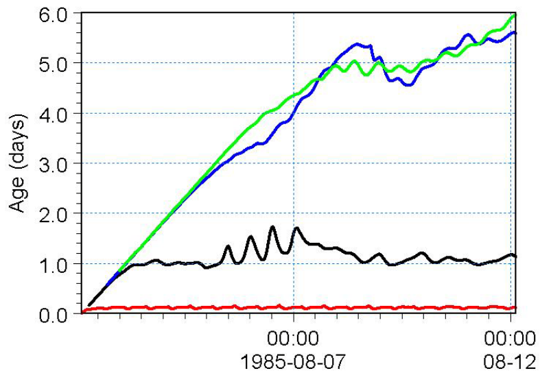
Figure 4.4 Age at four stations. Red line: point 1, black line: point 2, blue line: point 3 and green line: point 4. The locations for the points are shown on Figure 4.1.
