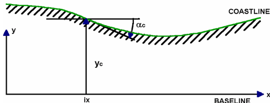
Figure 5.20 Coordinate system in coastline evolution model
