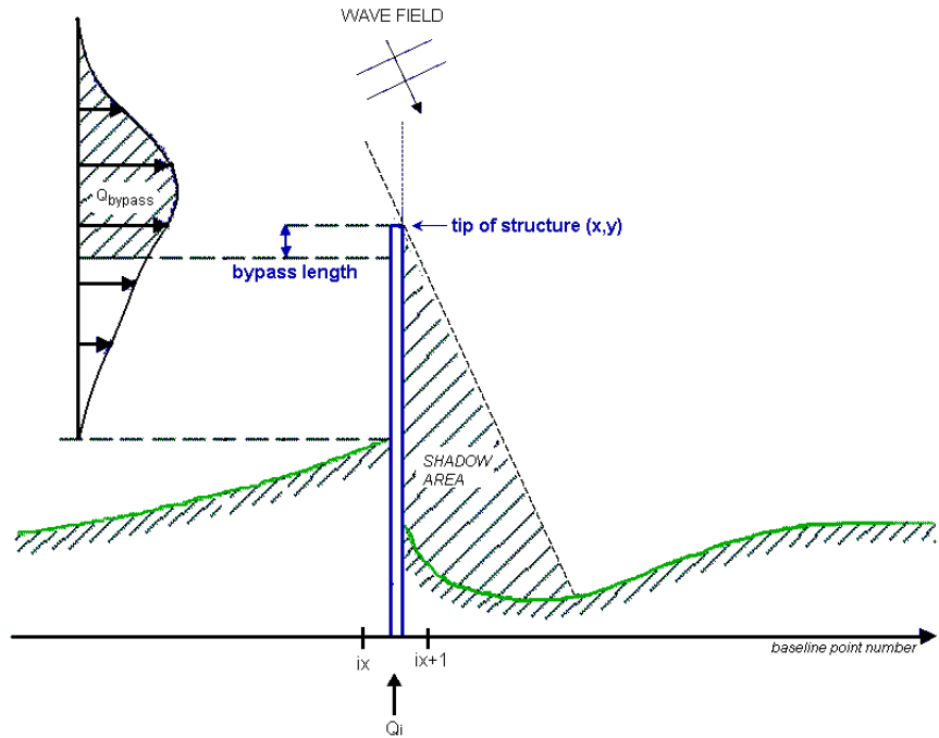
Figure 5.14 Definition of groyne
