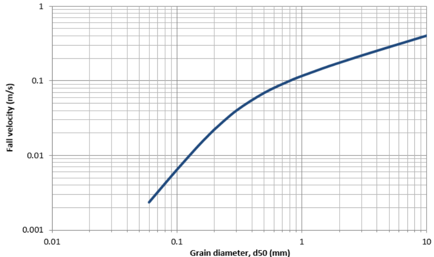
Figure 5.11 Fall velocity for uniform sediment by a water temperature of 12°C
