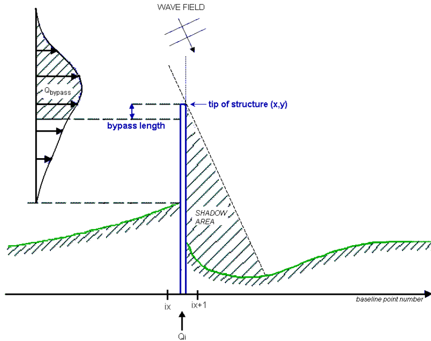
Figure 5.15 Definition of jetty
