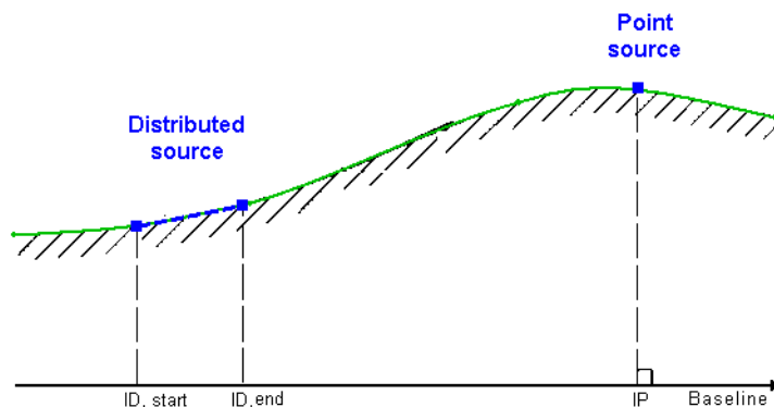
Figure 5.18 Definition of source location
