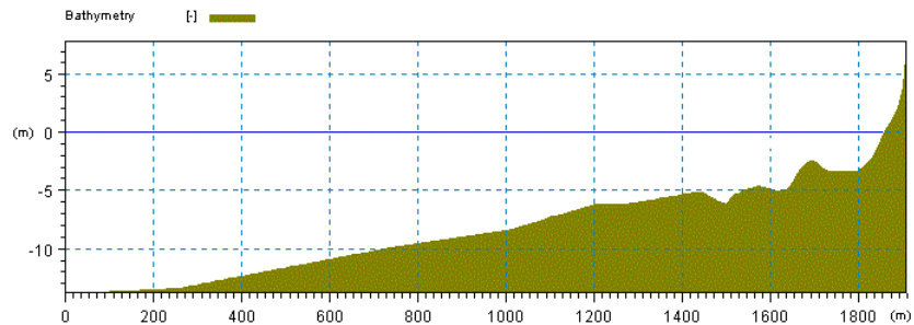
Figure 5.2 Example of cross-shore profile bathymetry
