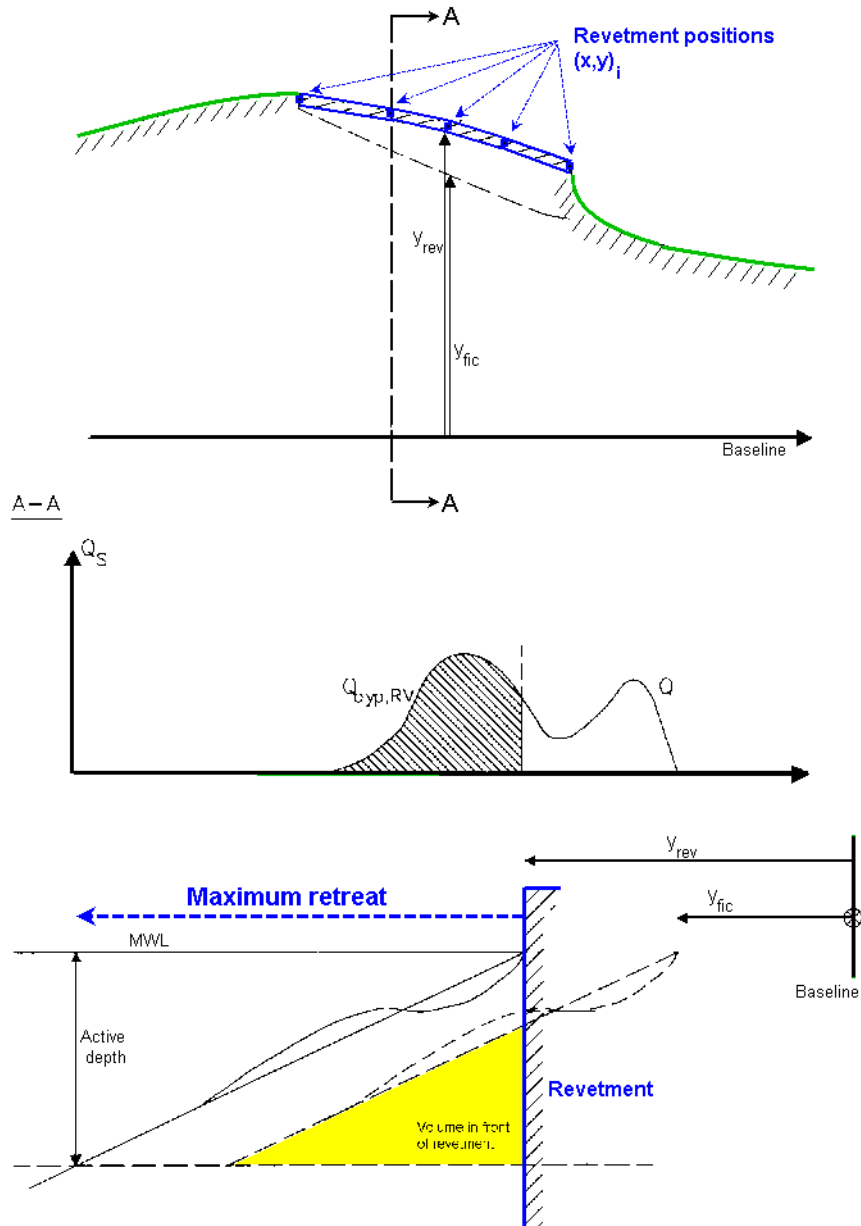
Figure 5.17 Definition of revetment
