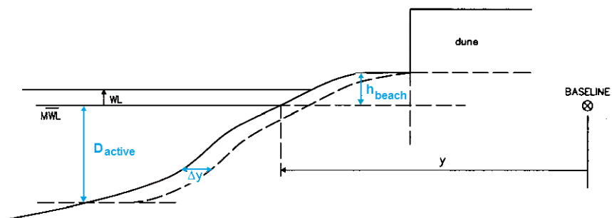
Figure 5.23 Definition of active profile height and initial movement of coastline
