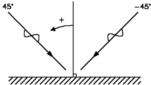
Figure 5.12 Definition of incoming wave angle in sediment transport tables
