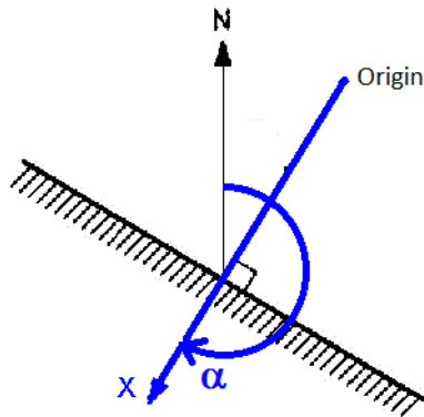
Figure 5.4 Definition of line orientation \alpha and cross-shore profile alignment
