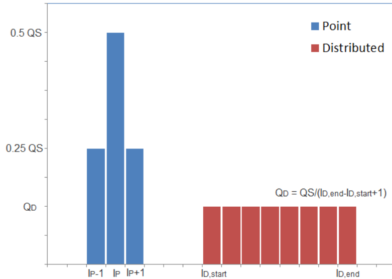
Figure 5.19 Distribution of sediment discharge from a point source and a distributed source, respectively, for the same source magnitude Q_S
