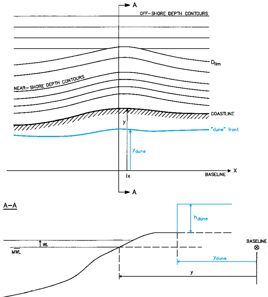
Figure 5.8 Definition of dune position and dune height
