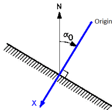
Figure 5.3 Definition of coastline orientation \alpha_0 and cross-shore profile alignment
