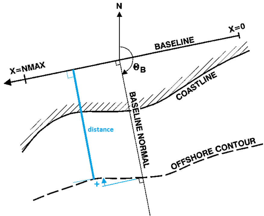
Figure 5.7 Definition of offshore contour position
