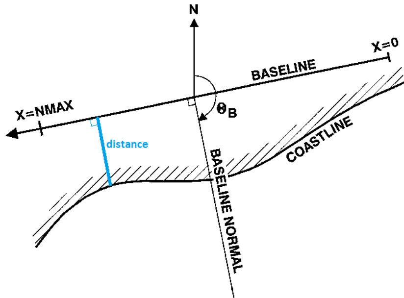
Figure 5.6 Definition of shoreline position
