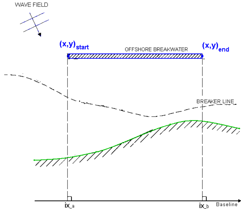
Figure 5.16 Definition of offshore breakwater
